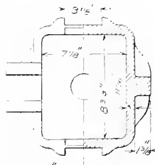
Fig. 4795. Plan of Body-bearing Casting.
